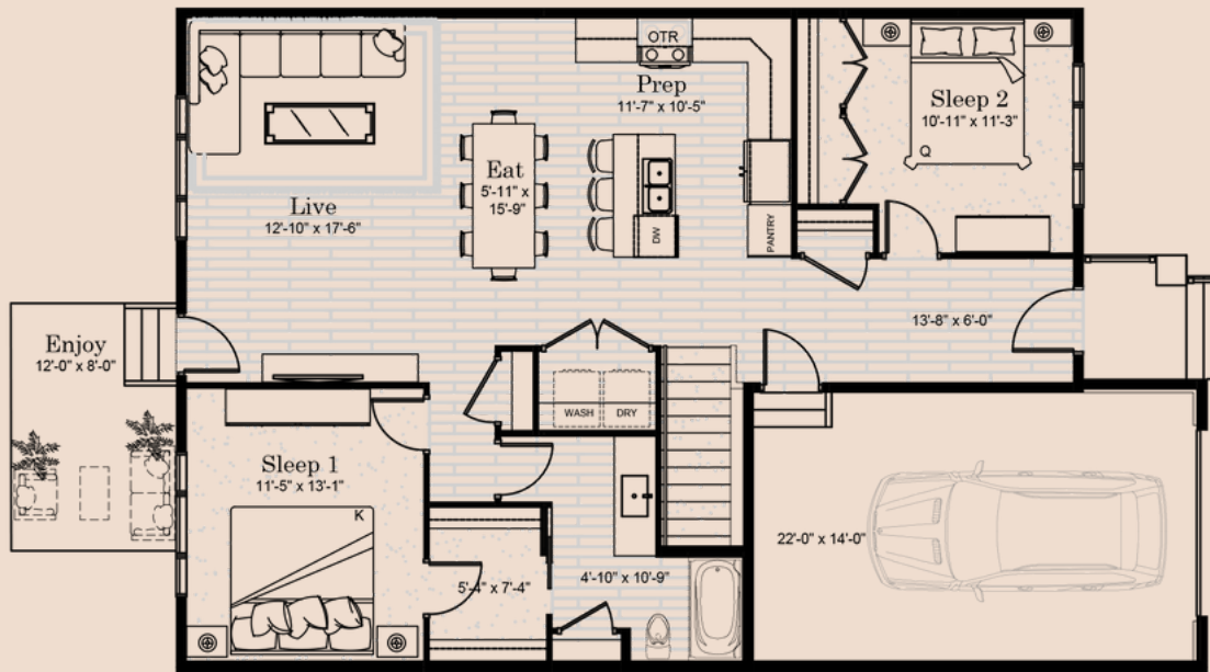
LOWER LEVEL - OPTIONAL DEVELOPMENT
